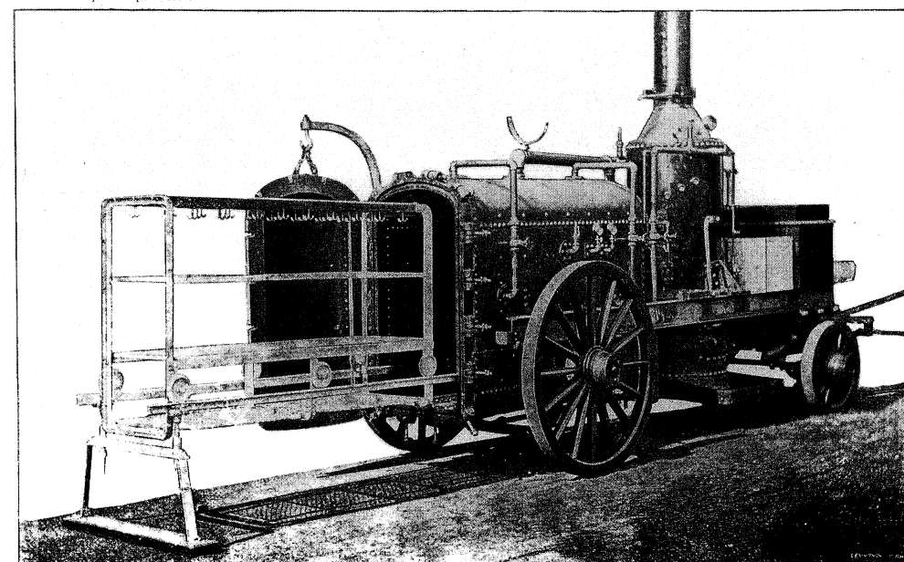
PORTABLE STEAM DISINFECTOR, KINYOUN-FRANCIS PATTERN, DESIGNED FOR U. S. MARINE-HOSPITAL SERVICE. "READY FOR SERVICE."
